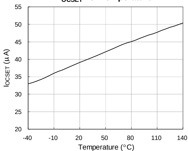
I OCSET vs. Temperature
