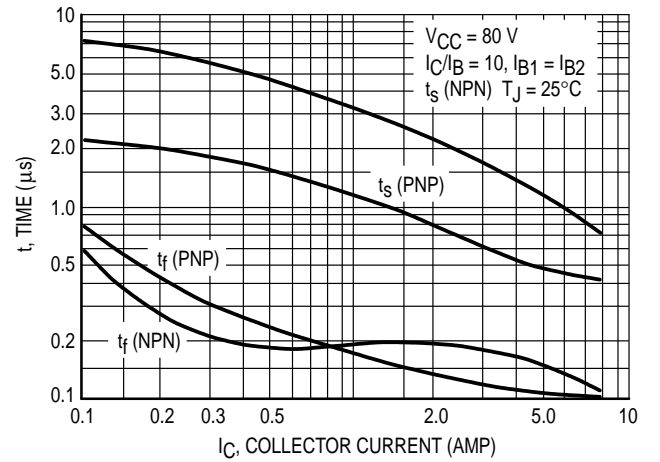
Figure 11. Turn-Off Times
