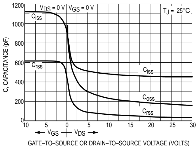
Figure 8. Capacitance Variation
