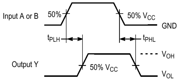
Figure 4. Switching Waveforms
