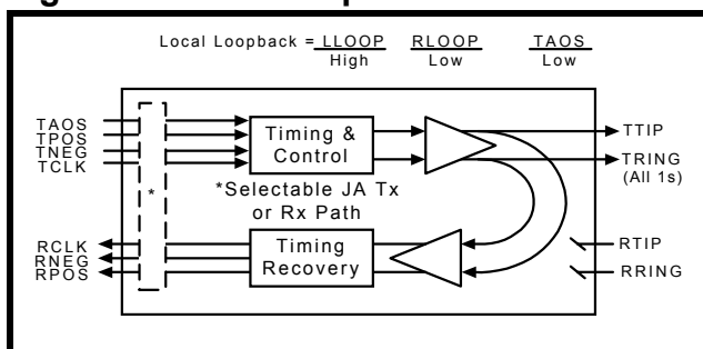
Figure 8: Local Loopback
