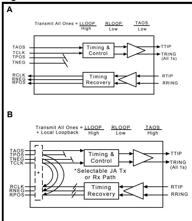
Figure 8: Local Loopback
