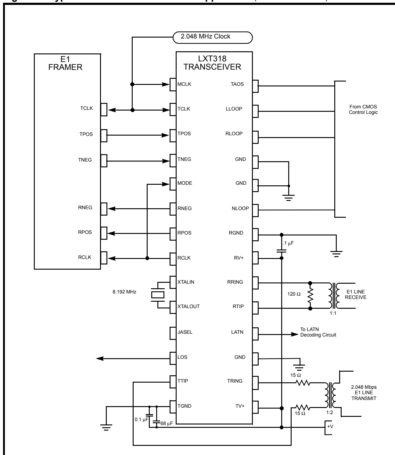
Figure 12: Typical LXT318 Hardware Mode Application (120 \Omega Twisted Pair)
