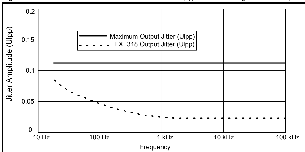
Figure 21: LXT318 Jitter Attenuation Performance (Typical—Measured Against TBR12/13)
