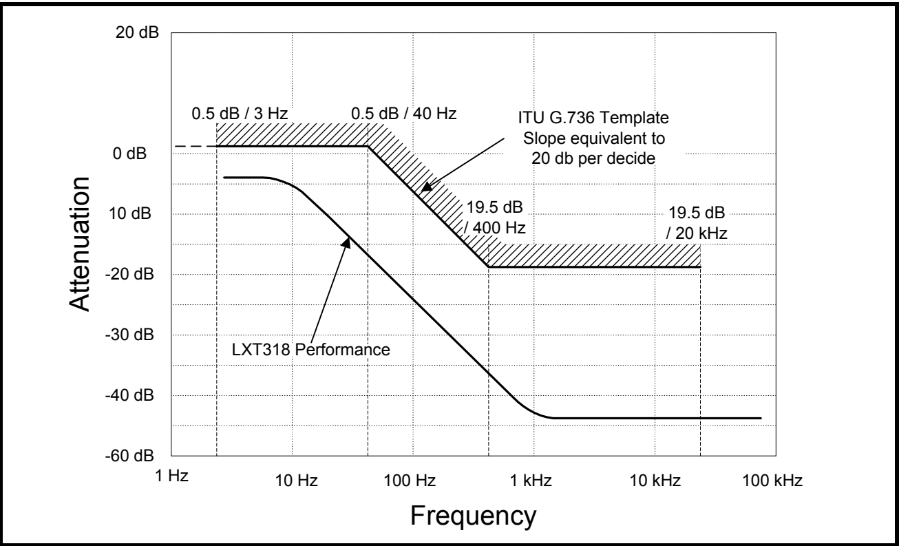
Figure 19: LXT318 Jitter Attenuation (Typical)
