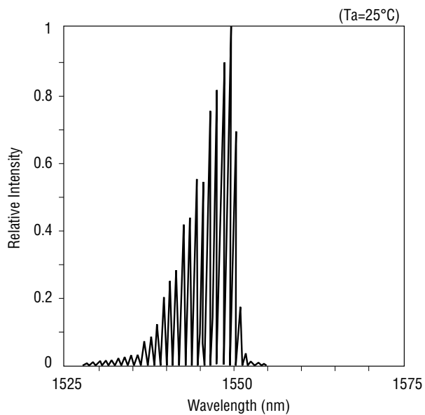
Oscillation Spectrum
