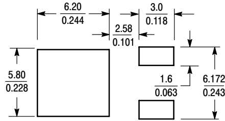
DPAK SCALE 3:1 (mm/inches)
