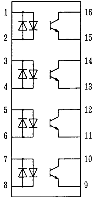
Pin Nos. and internal connection diagram
