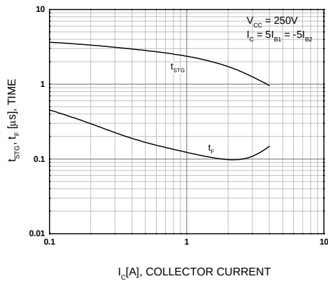
Figure 5. Resitive Load Switching Time
