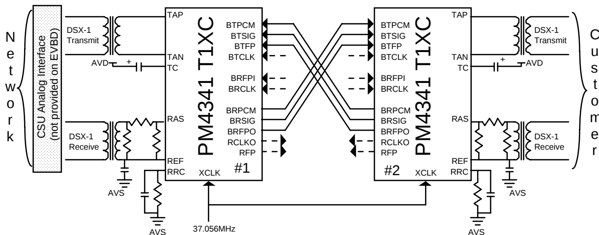
Figure 2: Jitter Attenuating "CSU" Application Hookup
