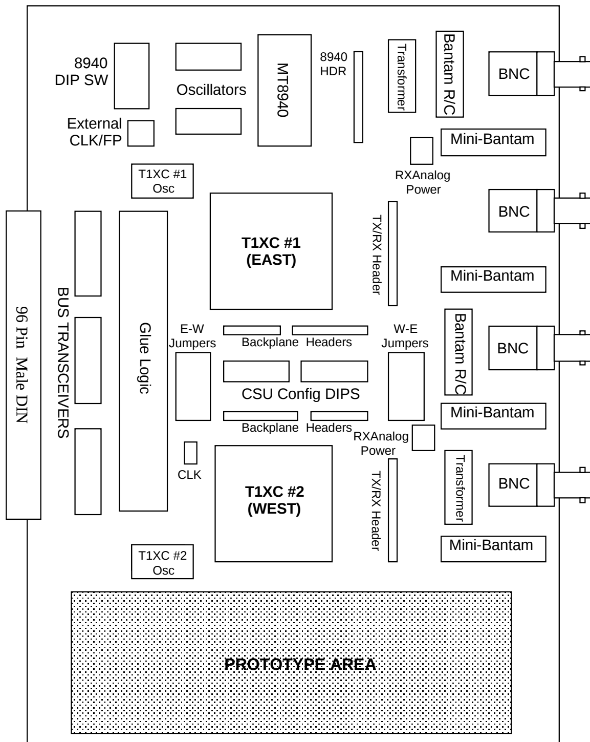
Figure 3: Board Layout
