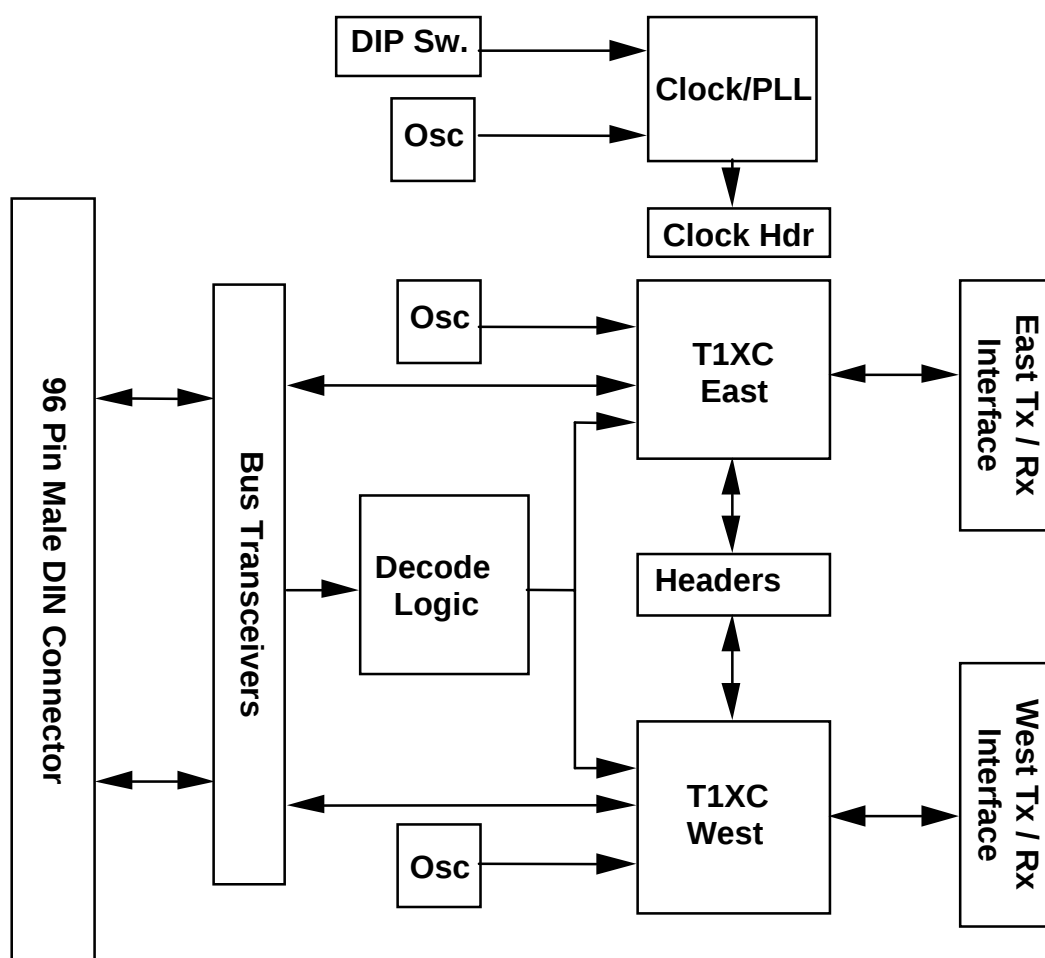
Figure 1: Block Diagram
