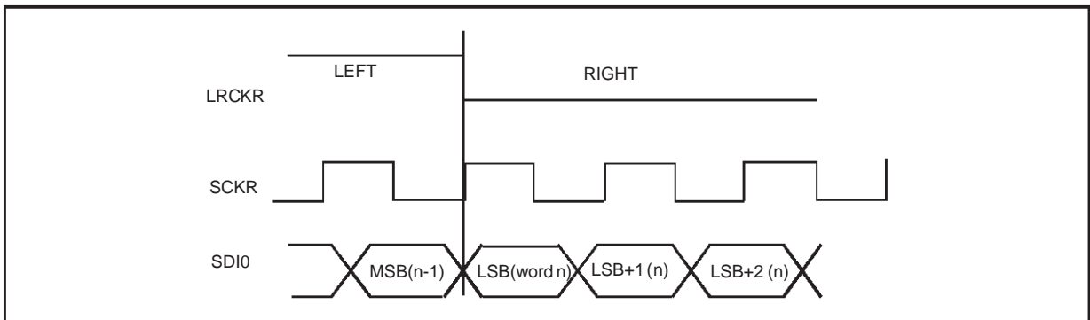
Figure 4. SAI protocol when RLR=1; RREL=0; RCKP=1; RDIR=1.
