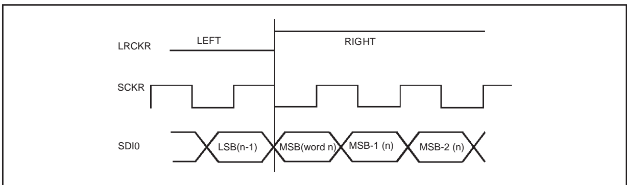
Figure 6. SAI protocol when RLR=0; RREL=1; RCKP=1; RDIR=0.
