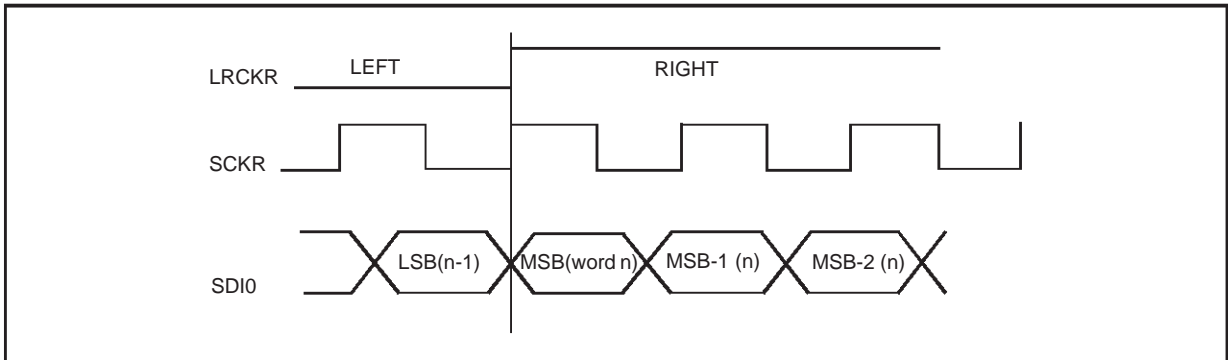
Figure 3. SAI protocol when RLR=0; RREL=0; RCKP=1; RDIR=0.
