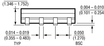
S Package 16-Lead Plastic Small Outline (Narrow 0.150) (LTC DWG # 05-08-1610)
