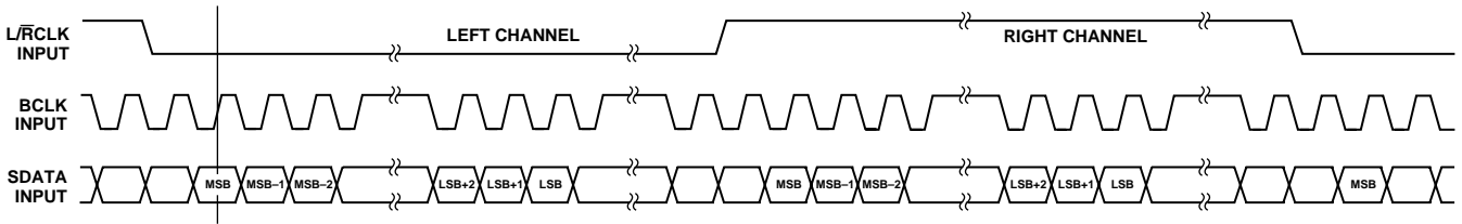
Figure 2. I2S-Justified Mode
