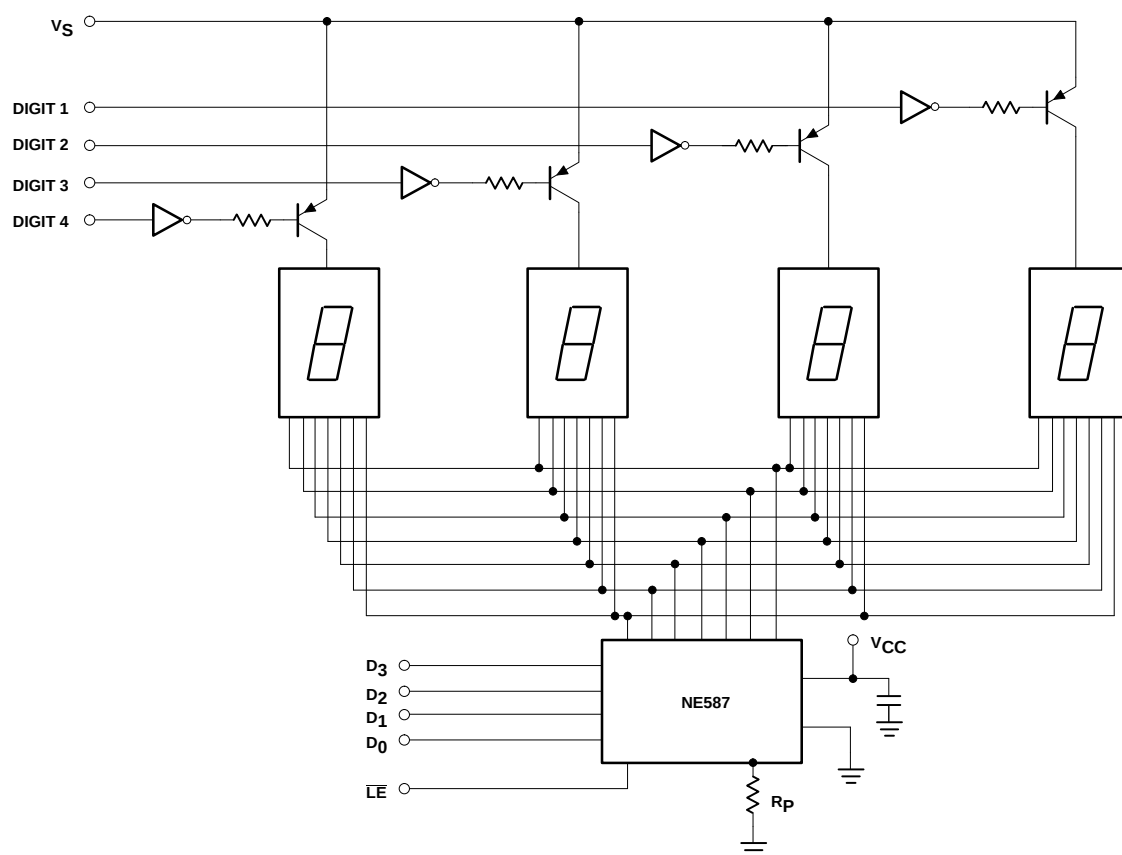
Figure 8. Interfacing 4-Digit Multiplexed LED Display
