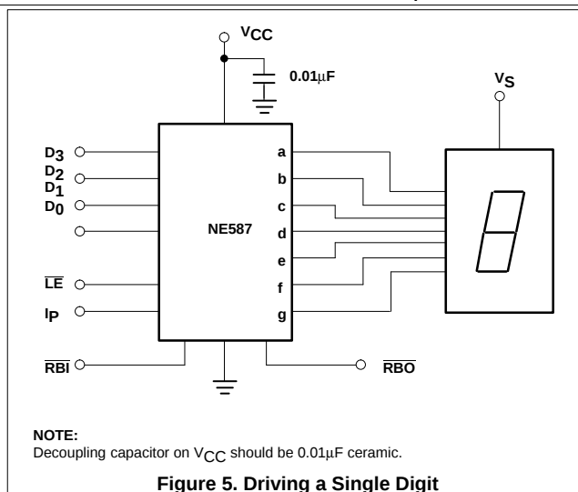
Figure 5. Driving a Single Digit
