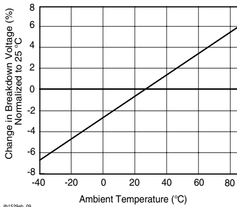
Figure 10. Switch Breakdown Voltage vs. Temperature
