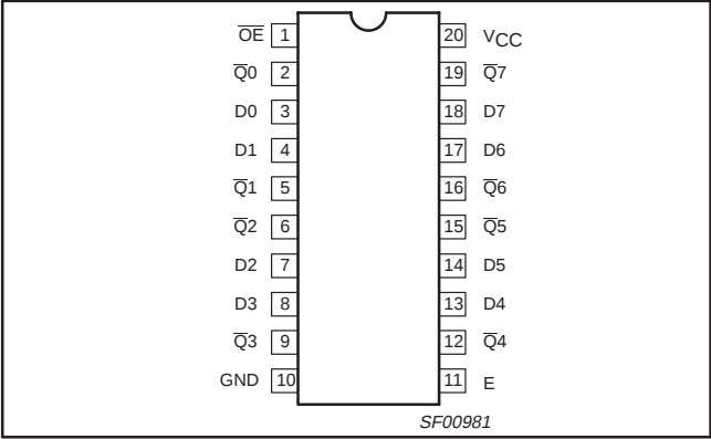
PIN CONFIGURATION – 74F533
