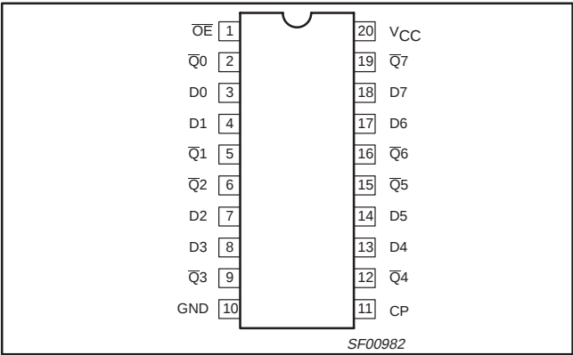
PIN CONFIGURATION – 74F534
