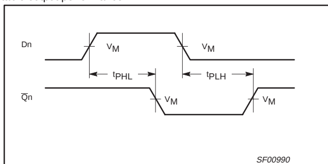
Waveform 2. Propagation Delay for Data to Output
