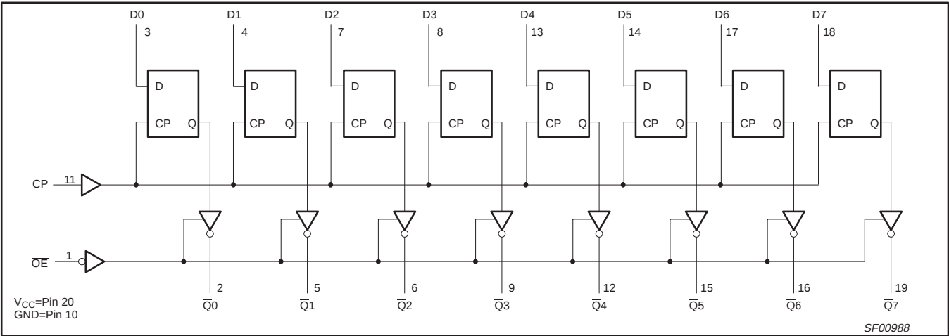
LOGIC DIAGRAM – 74F534
