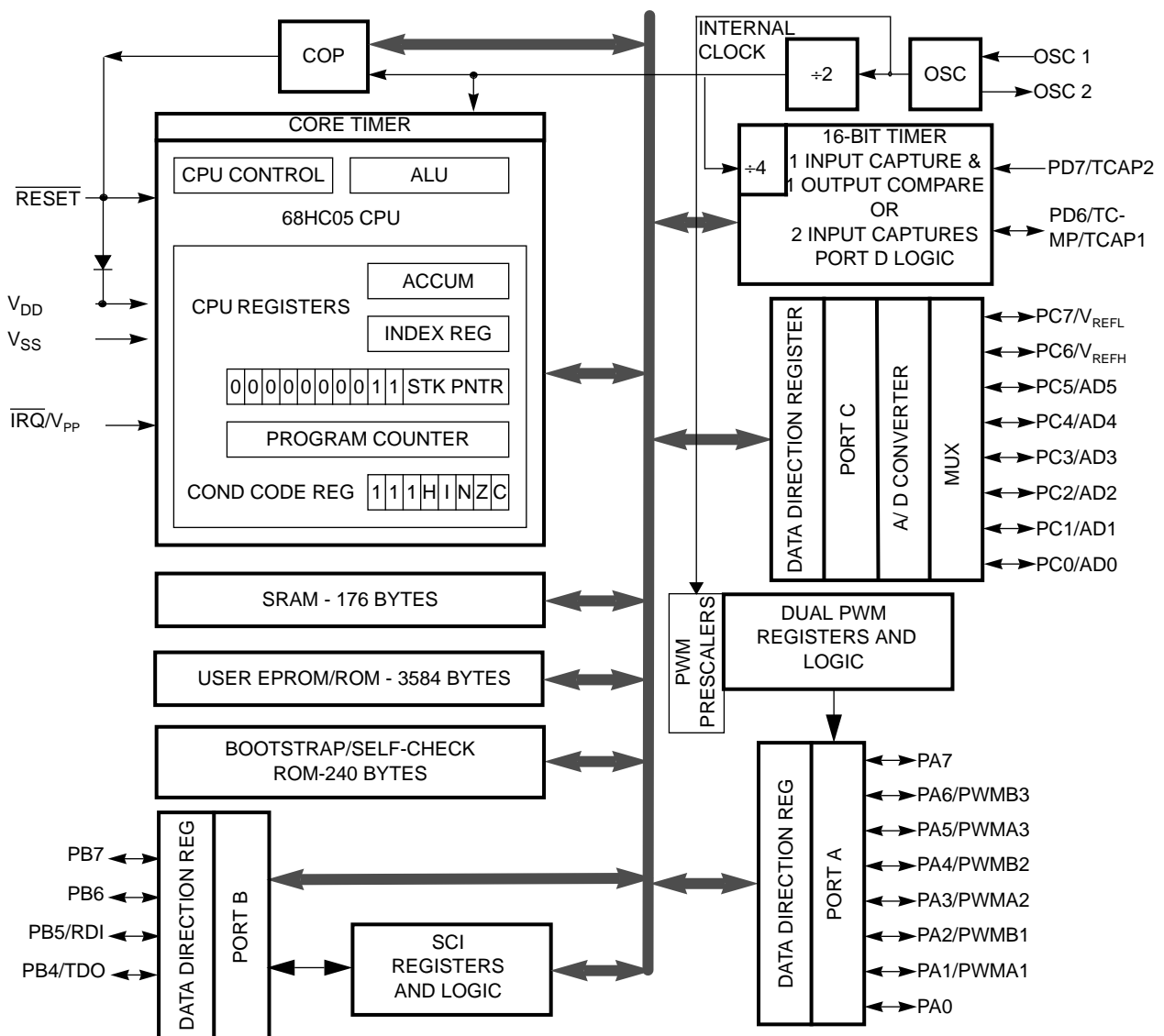
Figure 1-1: Block Diagram
