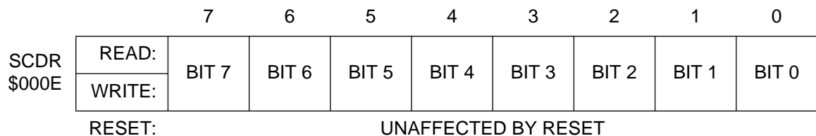
Figure 10-4: SCI Data Register (SCDR)
