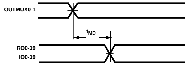
FIGURE 10. MULTIPLEXER TIMING
