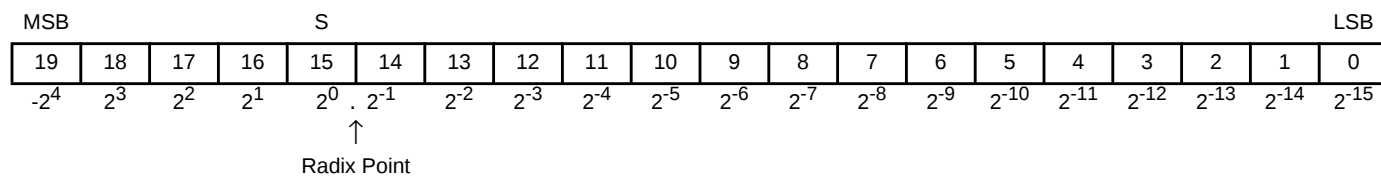
FIGURE 3. BIT WEIGHTING
