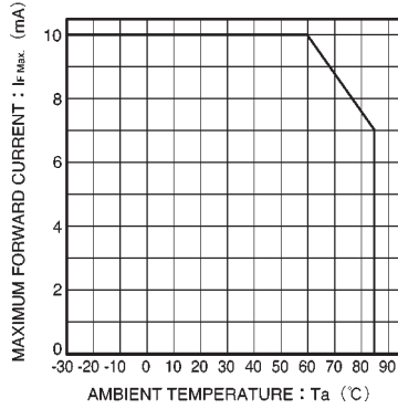
Fig. 6 Maximum forward current vs. ambient temperature
