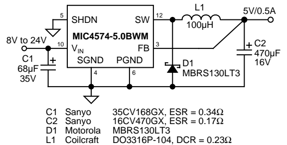
Figure 8. 8V–24V to 5V/0.5A Buck Converter Low-Cost Surface Mount
