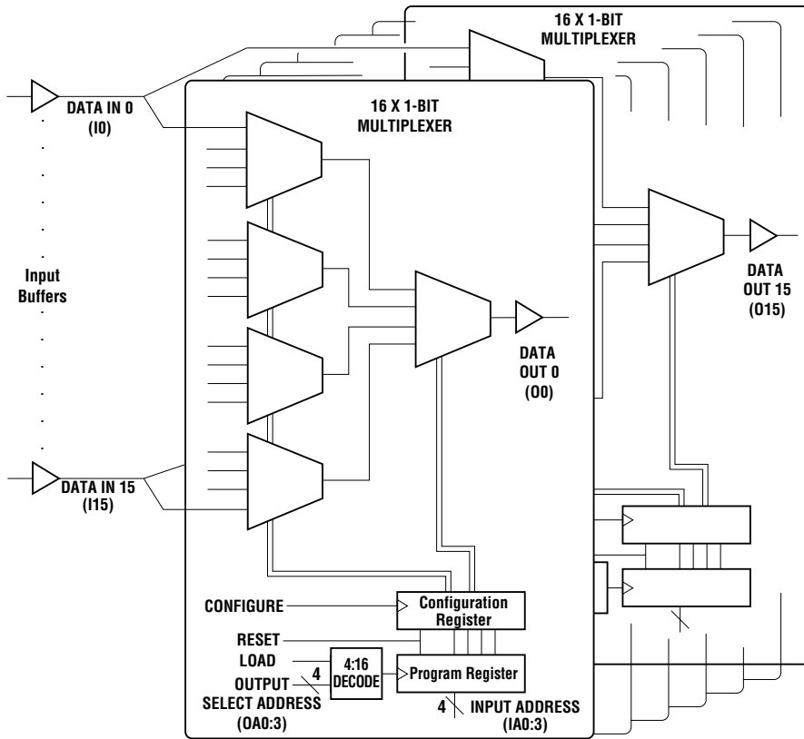
Figure 1. TQ8016 Architecture
