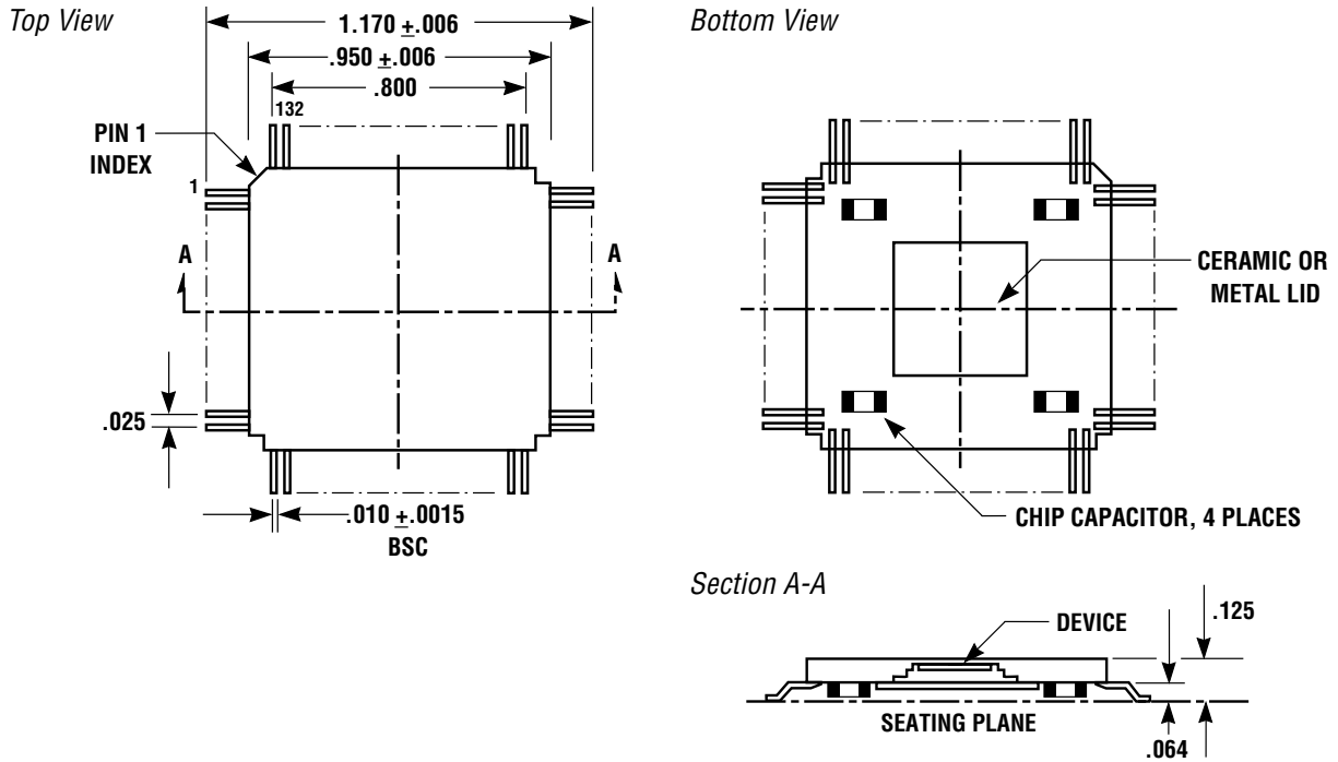
Figure 6. Mechanical Dimensions
