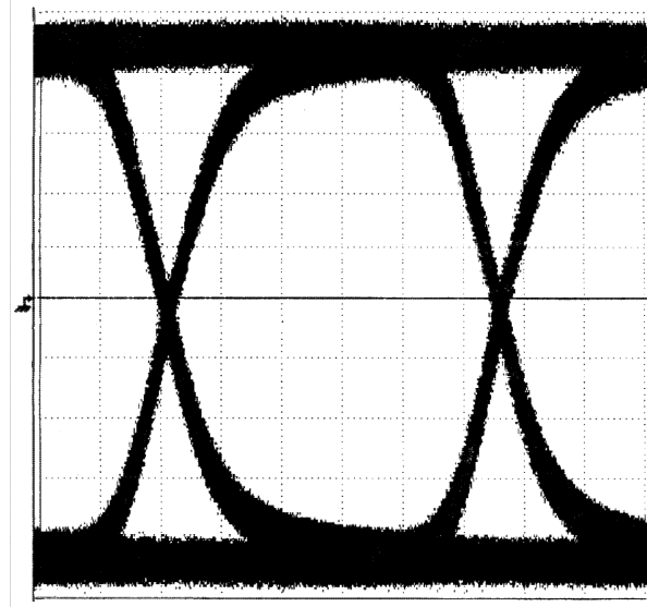
Figure 5. 1200 Mb/s Data "Eye" Pattern
