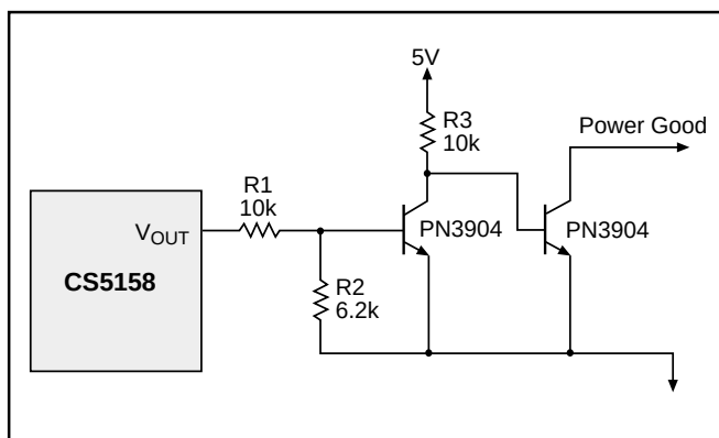
Figure 15: Implementing Power Good with the CS5158.
