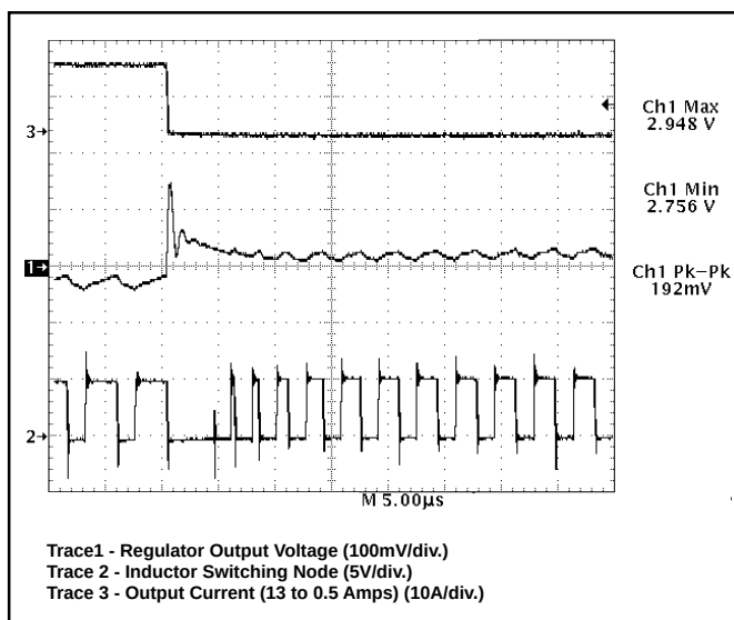
Figure 9: CS5158 demonstration board response to 13A load turn off (output set for 2.8V). V^2 ™ control topology immediately connects inductor to ground, providing 0% duty cycle. Regulation is achieved in less than 10µs.
