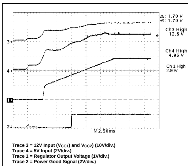
Figure 16: CS5158 demonstration board during power up. Power Good signal is activated when output voltage reaches 1.70V.
