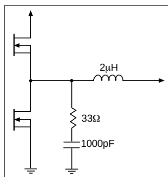
Figure 18: Filter components
