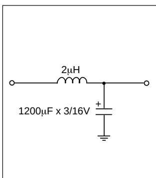
Figure 19: Input Filter
