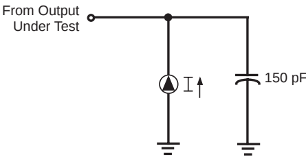
Figure 7. Test Load Diagram
