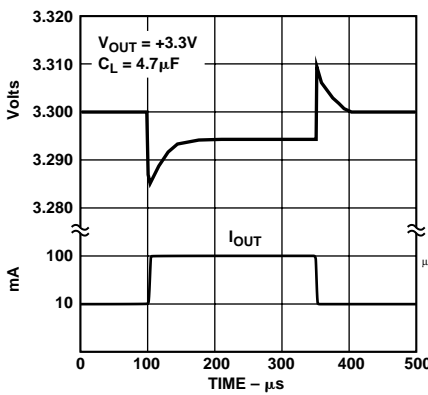
Figure 14. Load Transient
