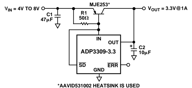
Figure 22. Higher Output Current Linear Regulator
